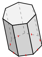
prisma heptagonal
