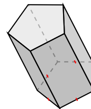
prisma pentagonal
