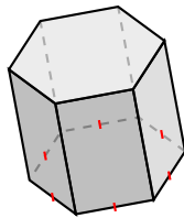
prisma hexagonal
