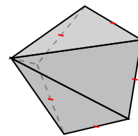
pentagonal pyramid
