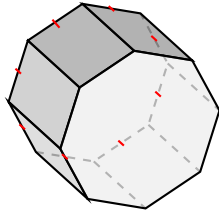
prisma octagonal
